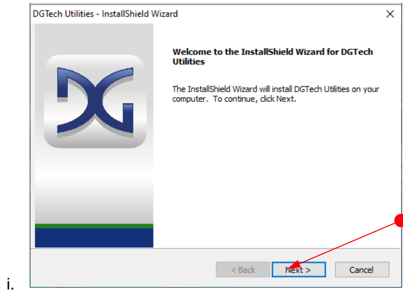
Figure 3 - Installation Welcome
