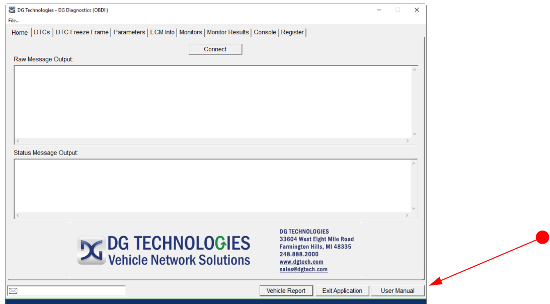
Figure 27 – Connection Screen
