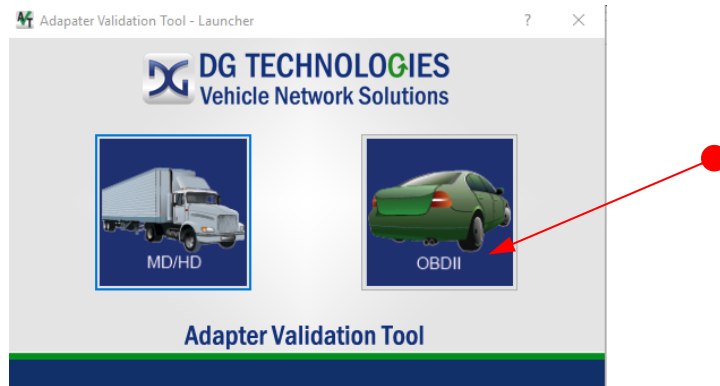
Figure 18 - AVT Startup
